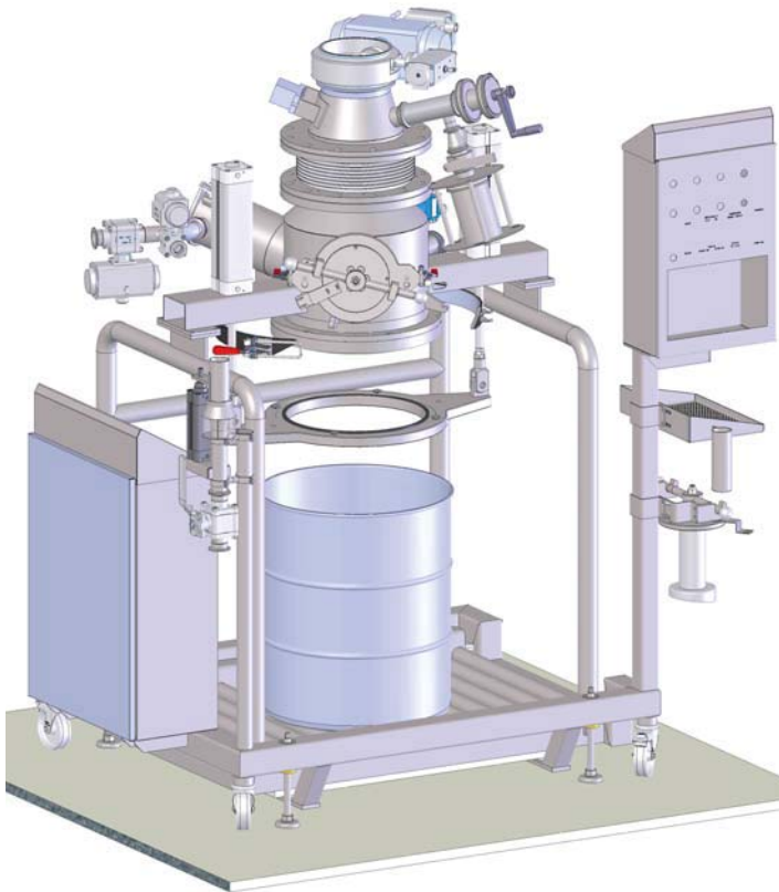
Contained WIP for single liner system
