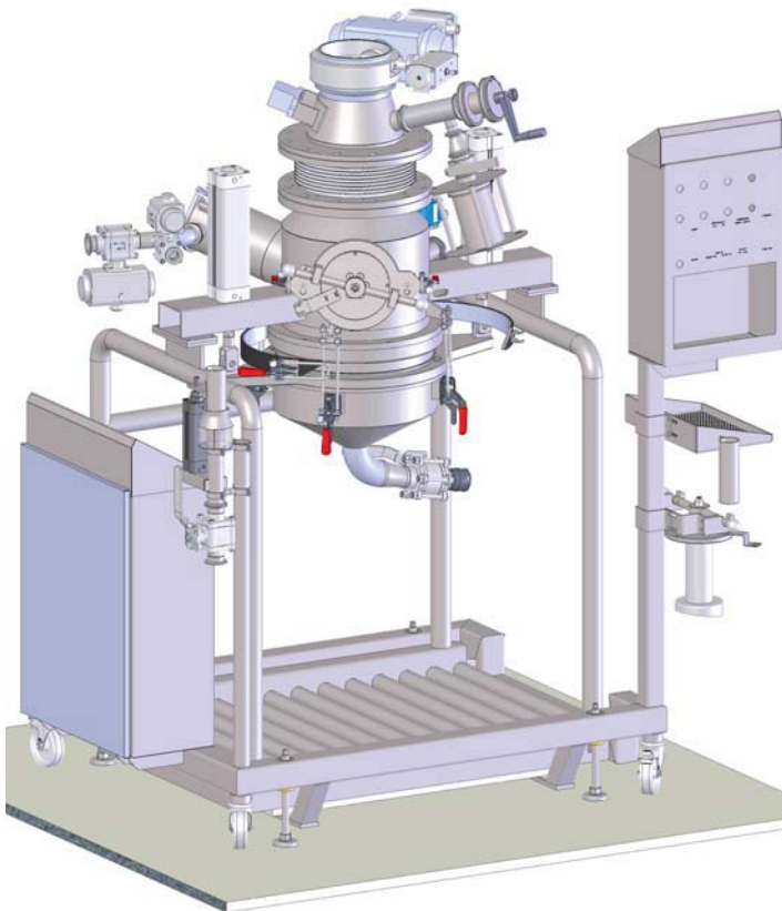
Contained WIP for single liner system
