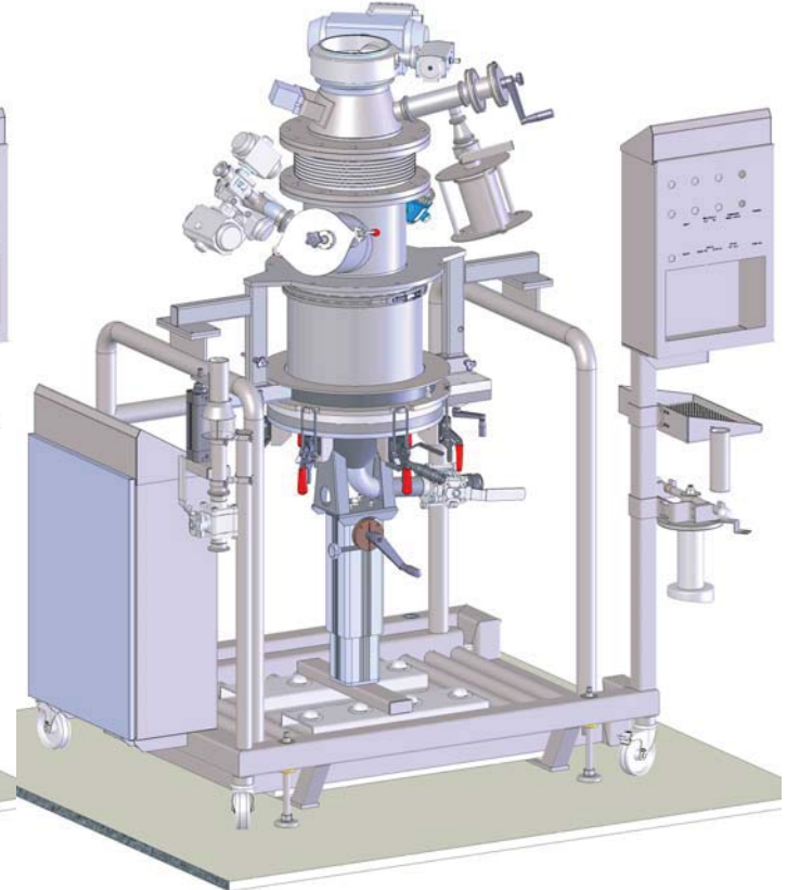
Contained WIP continuous liner system
